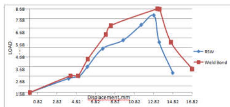
Fig: Load vs. Displacement
