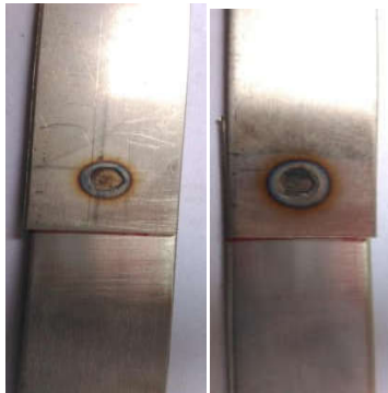
Fig: Resistance spot welding
