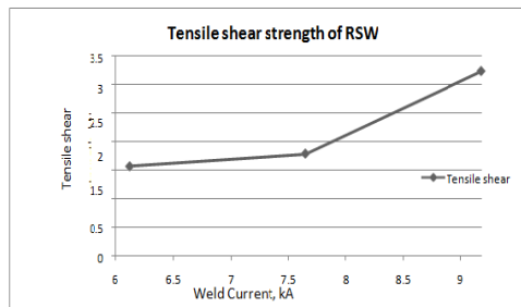
Fig: Tensile Shear strength of Resistance Spot Welding
