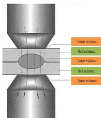
Fig: Resistance spot welding
