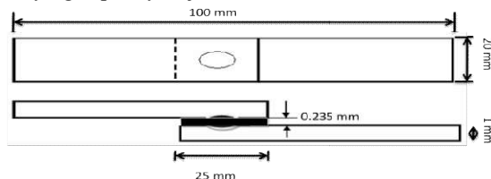
Fig: Specimen Geometry
